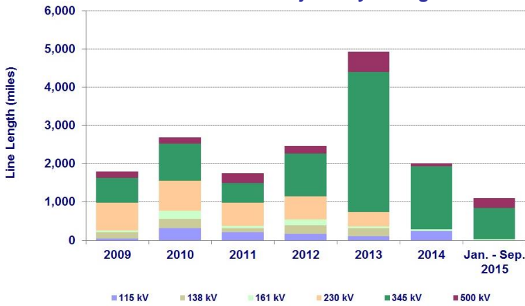
New Transmission Projects by Voltage
