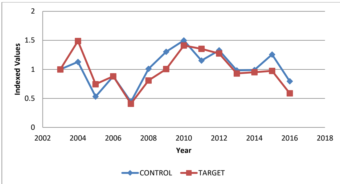
Figure 8. Total Irrigated Soybean Acres
