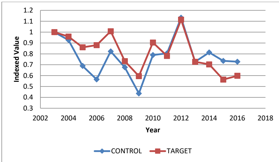
Figure 12. Average Groundwater Use per Irrigated Soybean Acre
