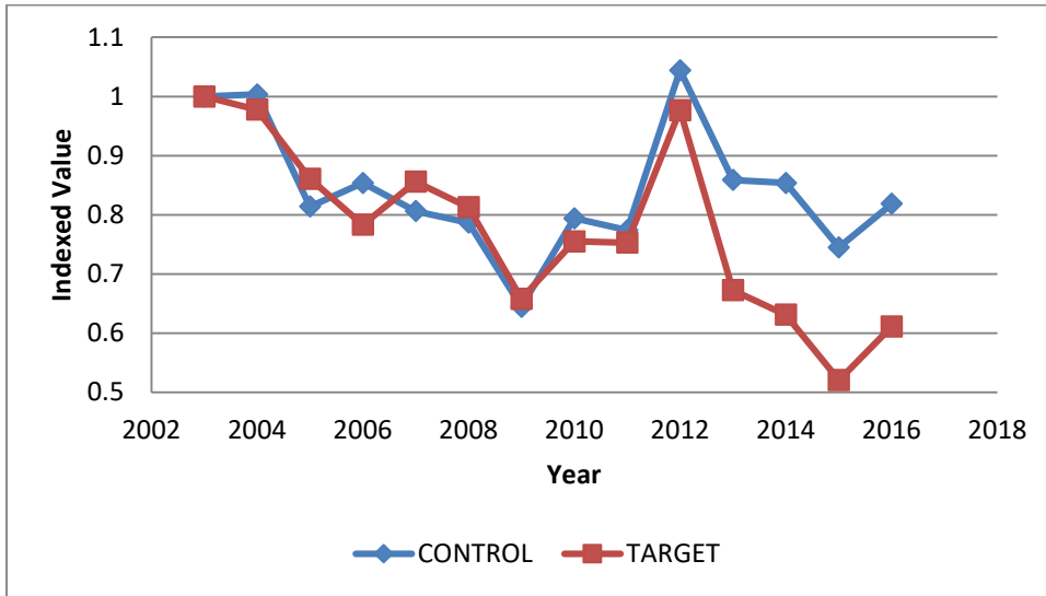
Figure 11. Average Groundwater Use per Irrigated Corn Acre
