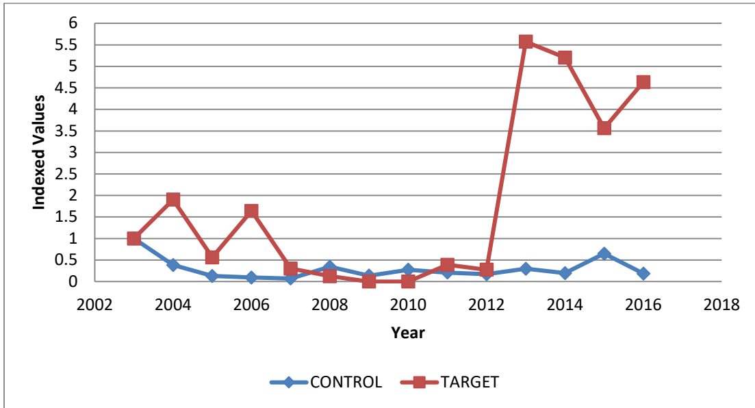
Figure 7. Total Irrigated Grain Sorghum Acres
